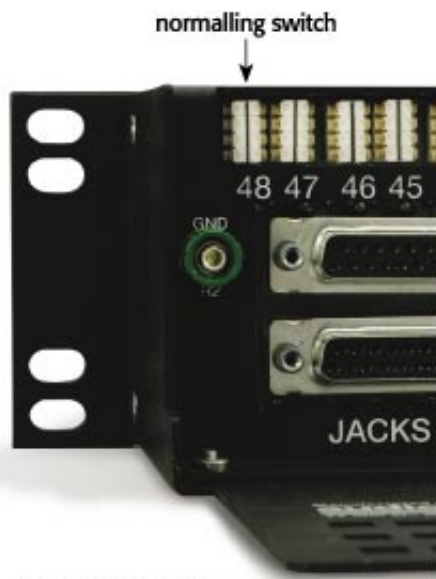
Rear view of patchbay.
